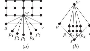
Figure 13: Counterexamples.
