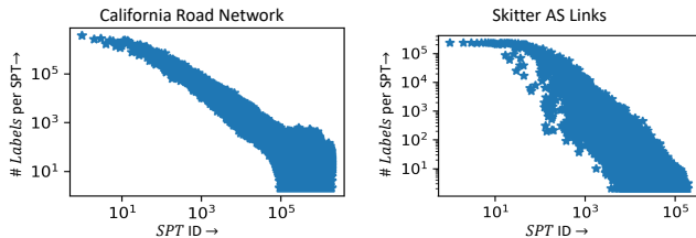
Figure 2: Labels generated by SPTs. ID of SPT_v is n - R(v) .
