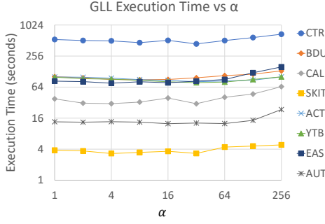
Figure 5: GLL execution time vs synchronization threshold \alpha
